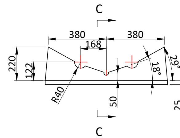
TRANSVERSAL SECTION "B"
