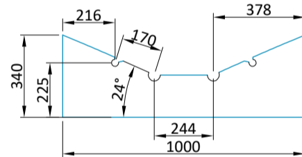
TRANSVERSAL SECTION "B"
