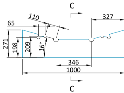
TRANSVERSAL SECTION "A"
