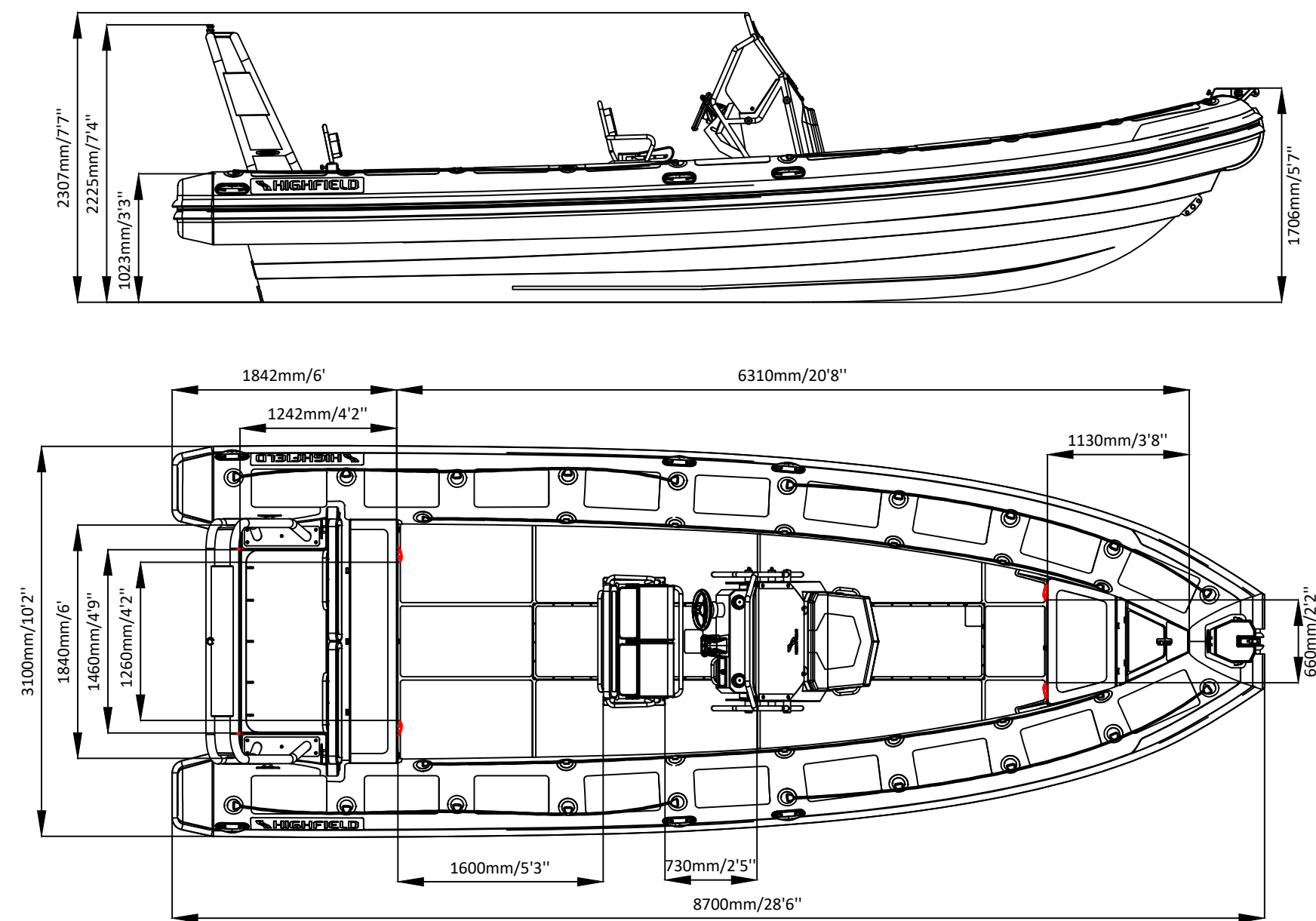
SPECIFICATIONS AND MAXIMUM CAPACITIES (Subject to change without notice.Tolerances:Dimensions ±2.5% Weight ±5%)
