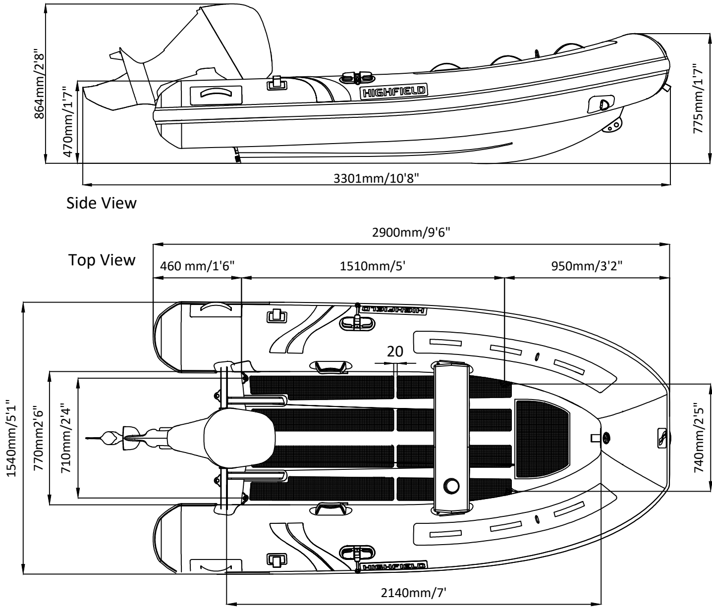
SPECIFICATIONS AND MAXIMUM CAPACITIES (Subject to change without notice.Tolerances:Dimensions ±2.5% Weight ±5%)
