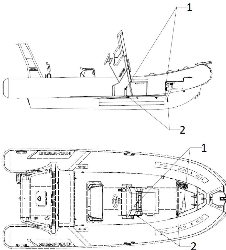
Diagram of the layout- Ventilation of petrol tank compartment
