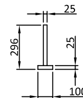
TRANSVERSAL SECTION "C"
