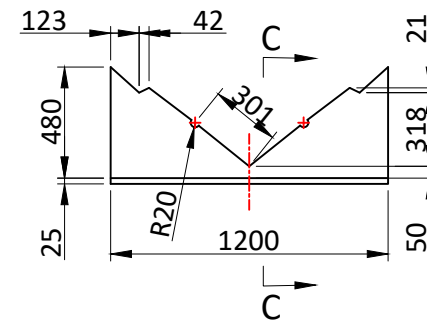
TRANSVERSAL SECTION "B"
