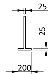
TRANSVERSAL SECTION "C"
