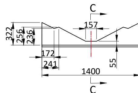
TRANSVERSAL SECTION "A"
