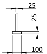
TRANSVERSAL SECTION "C"
