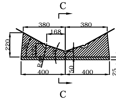
TRANSVERSAL SECTION "B"
