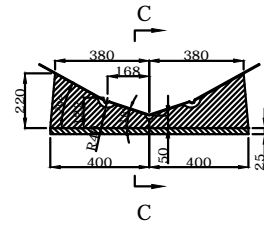
TRANSVERSAL SECTION "B"
